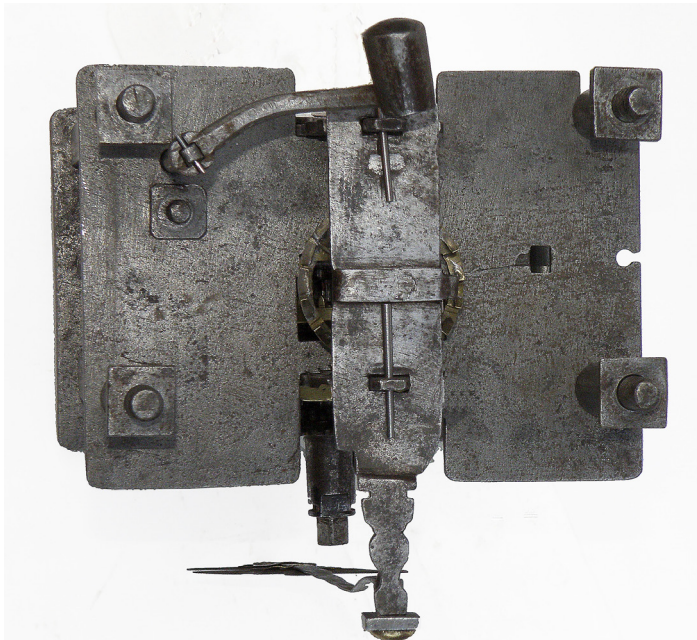
Movement from the front showing the vertical hammer shaft.
