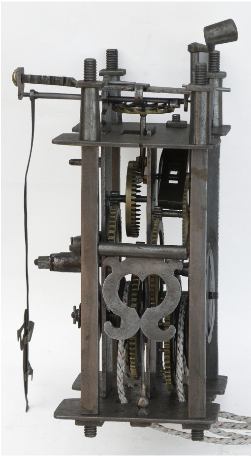
Right-hand side showing the single arbor for the strike-work and the large decorative trip lever.
