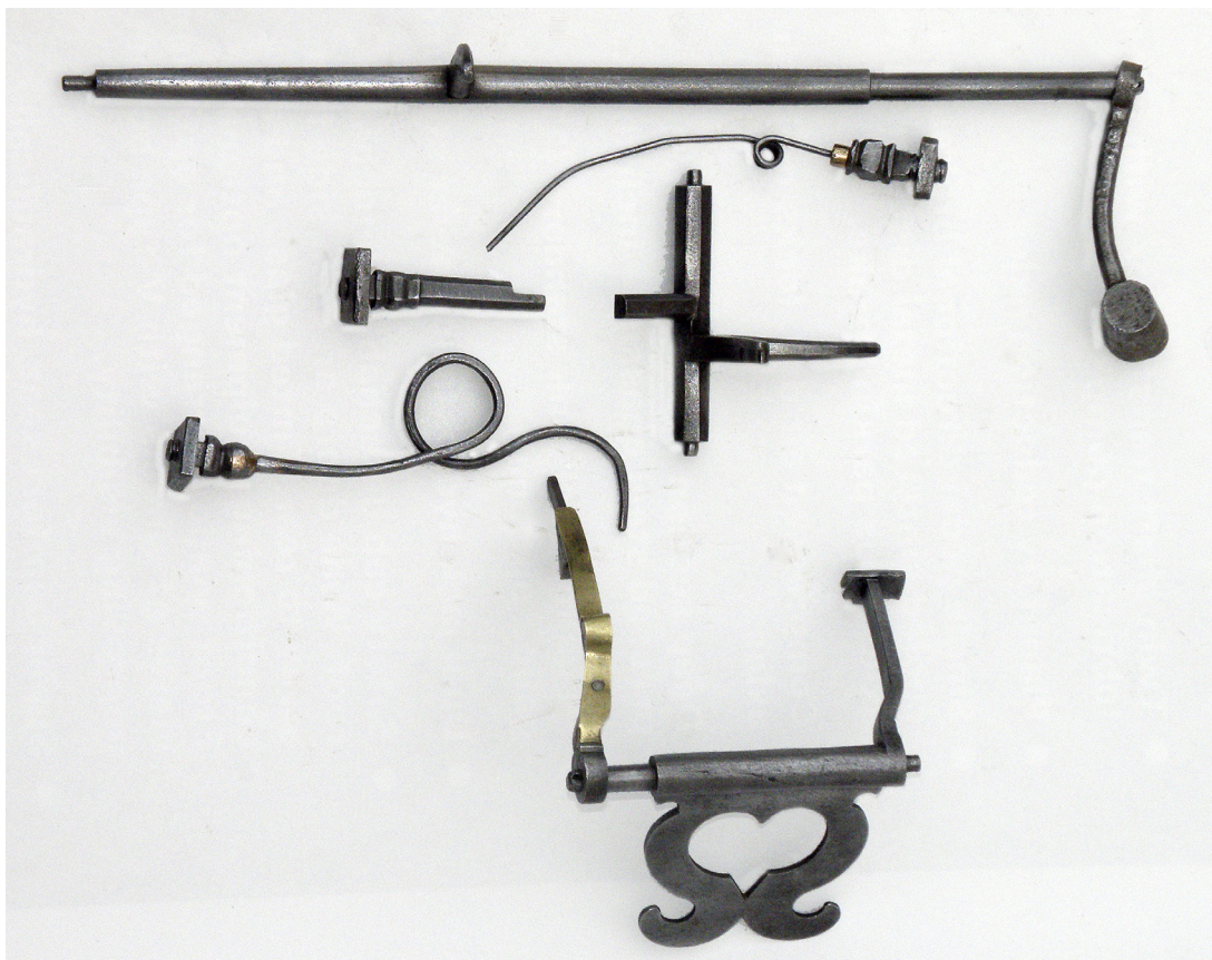
The components of the strike-work, all of iron apart from the brass return spring of the nag's head. The seemingly simple locking detent also acts as an overlift lever and countwheel detent.
